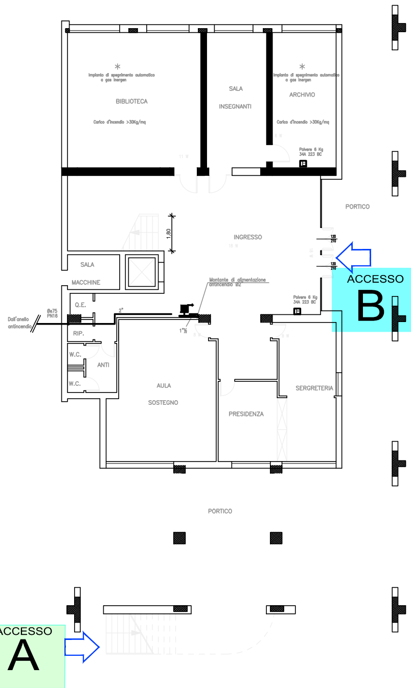
PIANO TERRA
